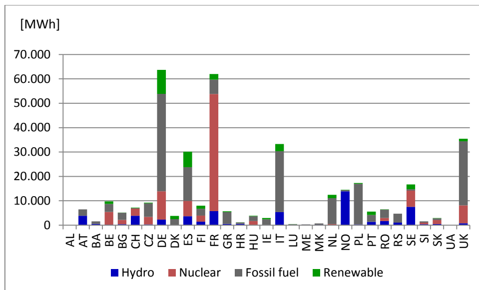
Figure 34: Average generation in 2011 based on ENTSO-E
