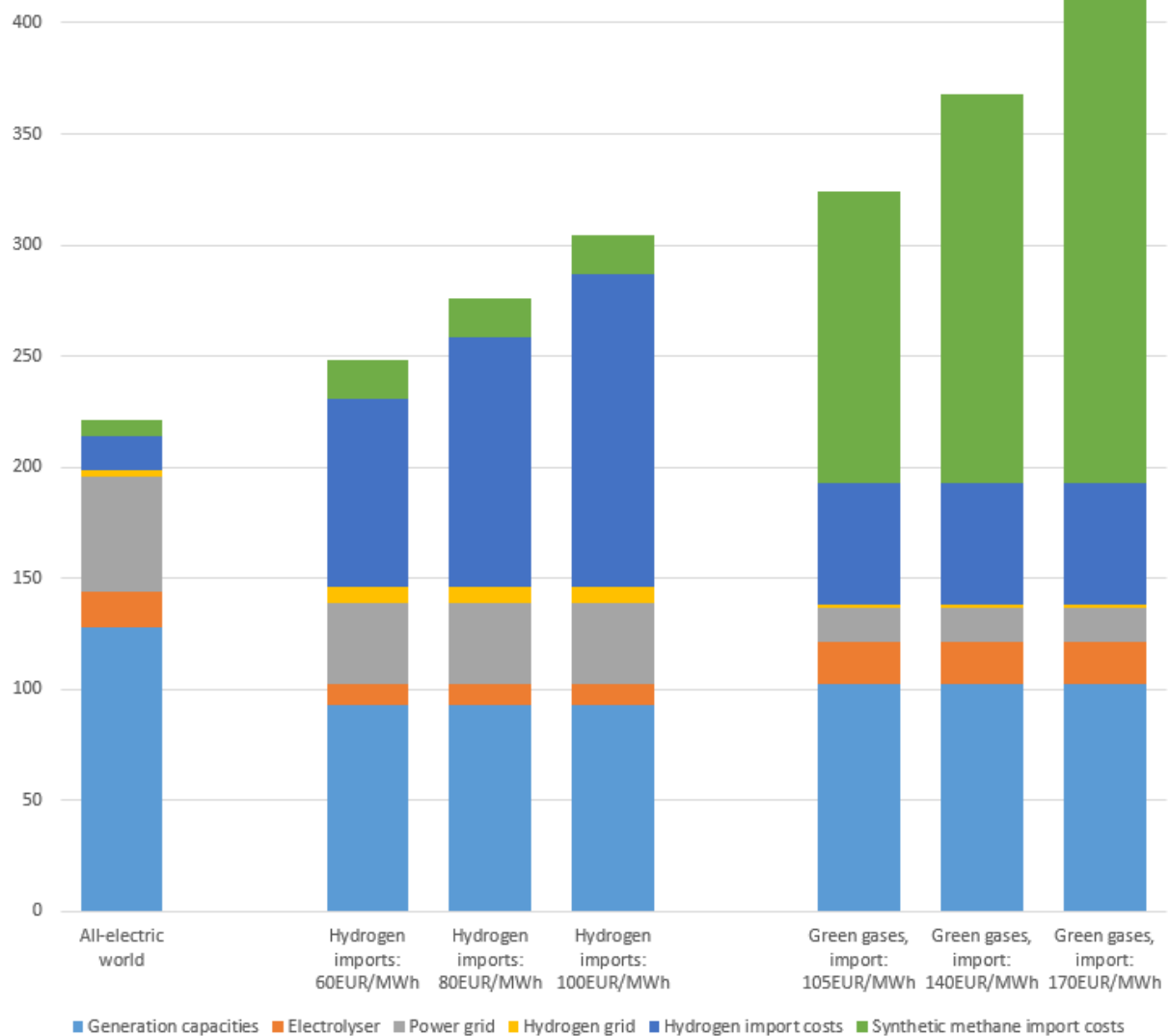
Figure 6-5: Annual system costs sensitivity to import prices
