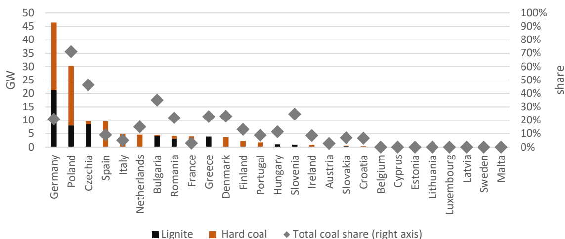
Figure 3-10: Installed capacity in MW of coal-fired power plants in 2019
