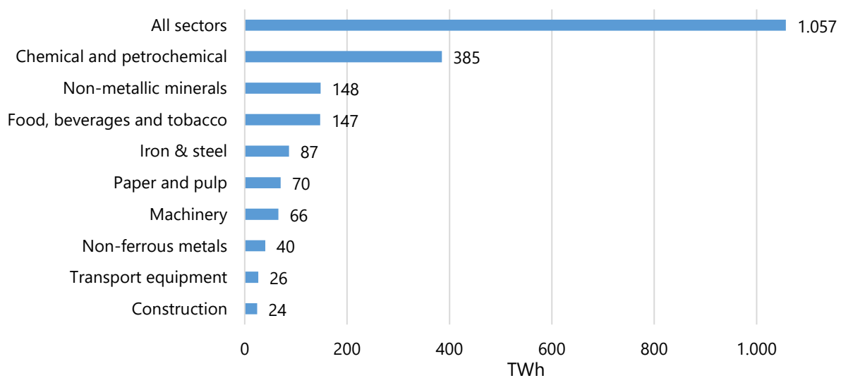
Figure 4-7 Industrial usage of fossil natural gas
