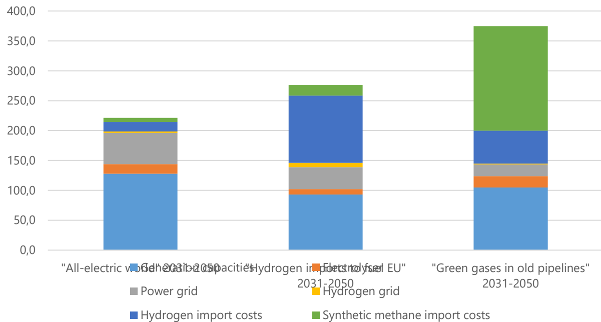
Figure 6-4: Average annual investments and fuel import costs
