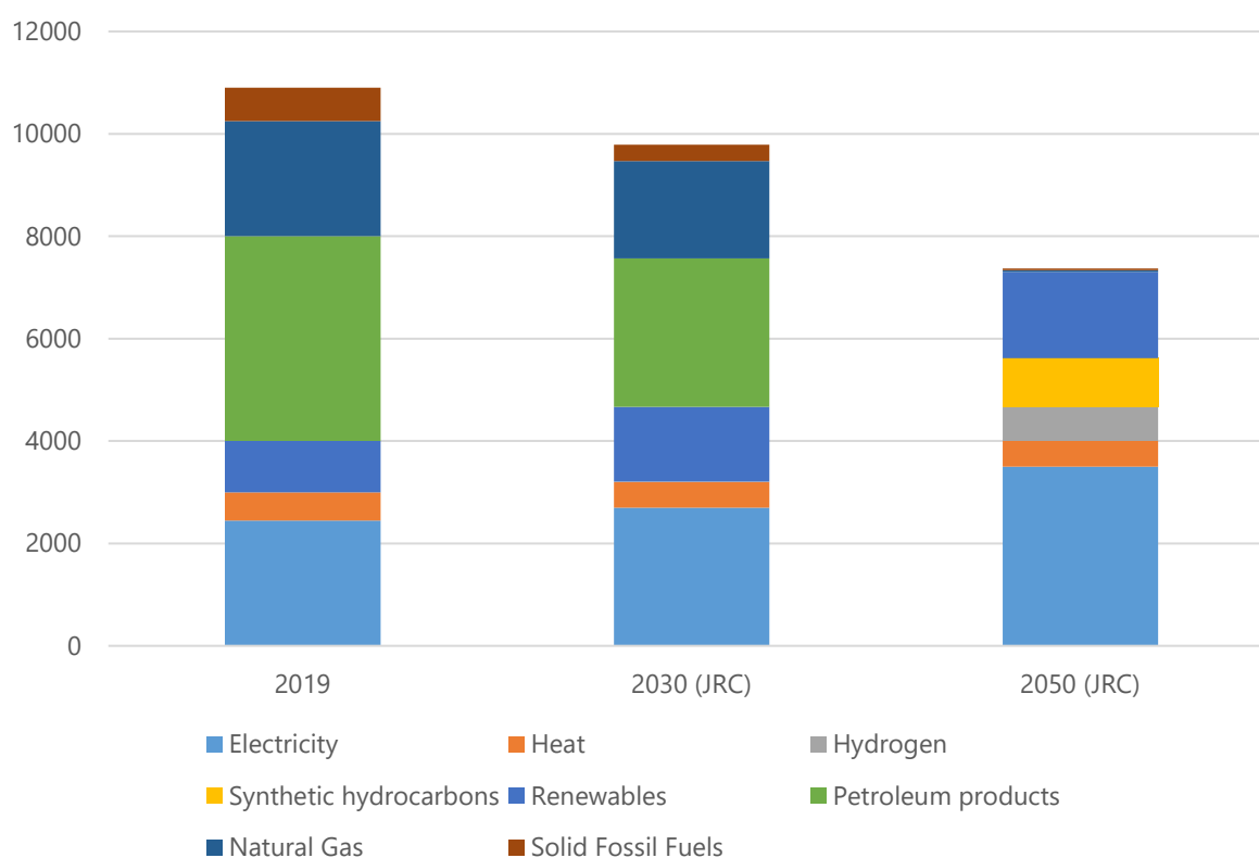
Figure 2-1: JRC Final Energy Consumption by Fuel (TWh)
