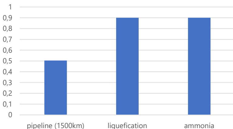
Figure 5-4: Additional transport costs (€/kg)
