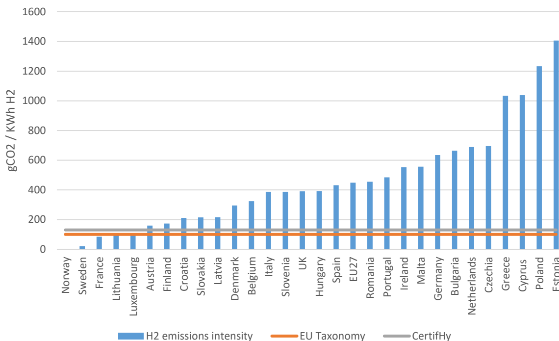
Figure 5-6: Electrolytic hydrogen from average grid intensity
