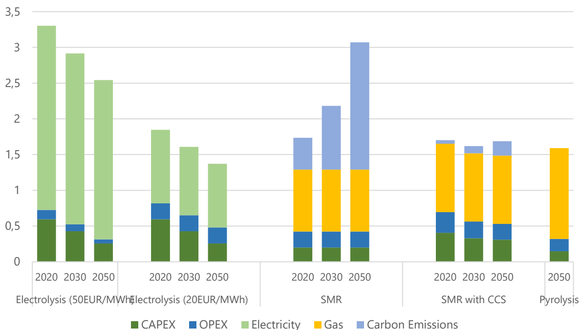
Figure 5-3: Hydrogen Production Cost Decomposition (EUR/kg)
